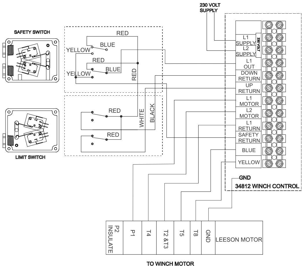
Figure 2. Wiring Diagram.
