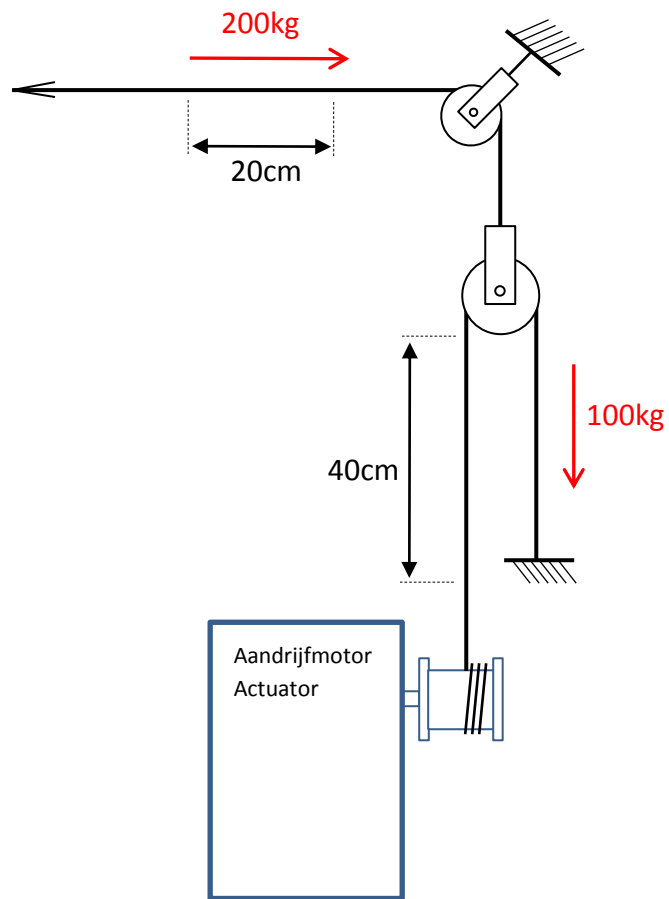
Inscharen Movable pulley system
