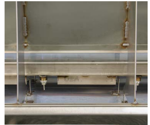
Chore-Time Shelf Feeder with removable water tube
